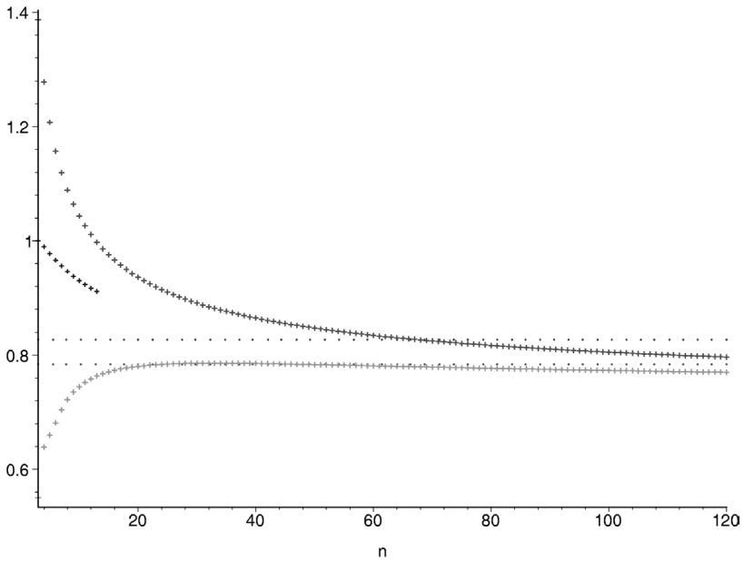
Fig. 1. The first values of \sqrt[12]{\alpha_n(12-34)/n!} between the lower and the upper bound given by Proposition 5.1.
