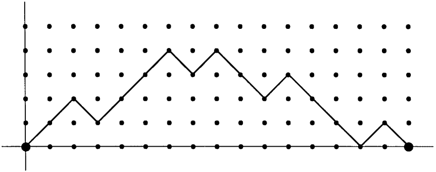
FIG. 1. The Dyck path corresponding to 74352681.
