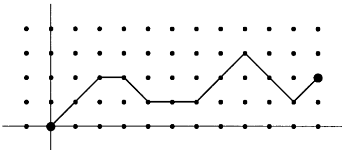
FIG. 2. A Motzkin path.
