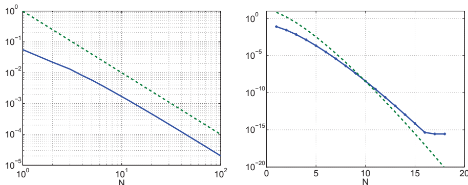
Fig. 3.1 Left: The approximation of \sqrt{\mathbf{K}_N} by a_{m-n} - a_{m+n} , with a_p from (3.9), and aliasing (3.12). We observe second-order accuracy (the dotted line has reference slope -2 ). Right: The approximation of \exp(-\mathbf{K}_N) via (4.4) and aliasing. The dotted line is Weideman's estimate of exponential accuracy (!) for a periodic integral [25]. We used MATLAB's sqrtn and expm as reference solutions. Both graphs show the largest error among the entries of the matrix.
